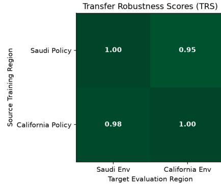
Figure 4: Cross-region Transfer Robustness Scores (TRS). Policies trained on one region are evaluated on the other. TRS \geq 0.95 indicates strong cross-region generalization.
